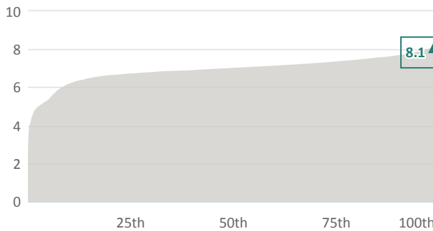
ESG QUALITY SCORE PERCENTILE VS. PEER GROUP EQUITY GLOBAL (N=5528)
